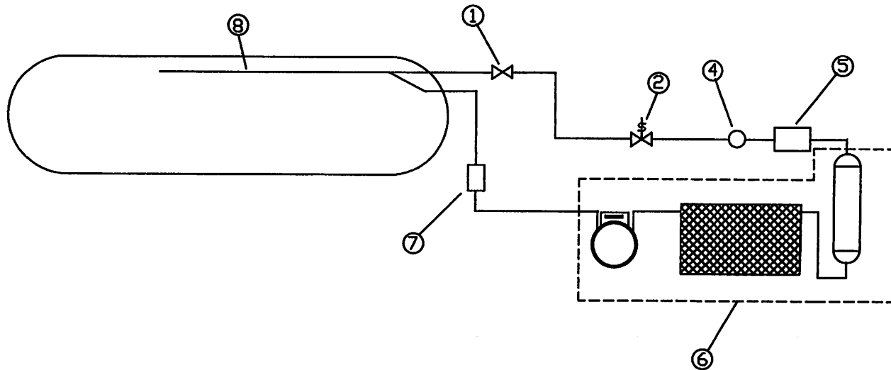
Refrigeration Schematic
