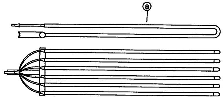
Coil Detail
