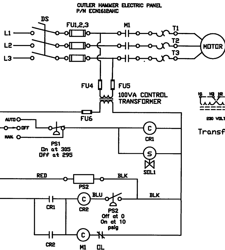
Electrical Schematic
